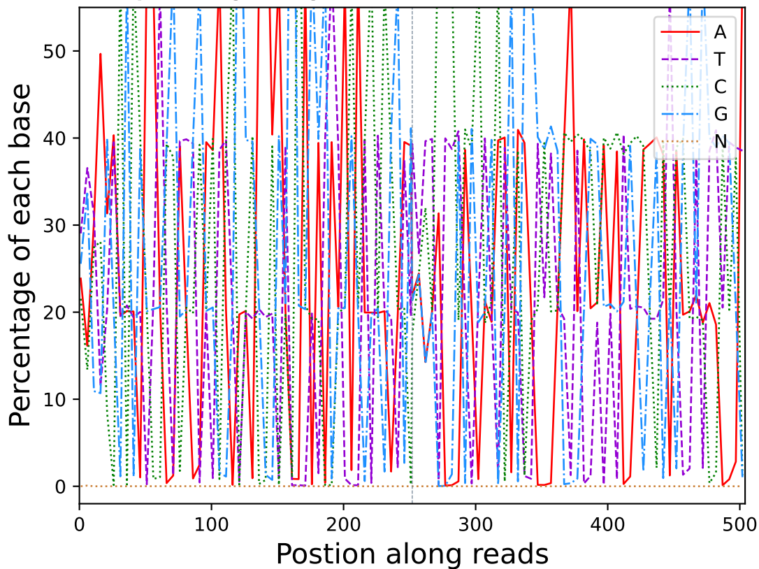
Base percentage along reads (R10730)
